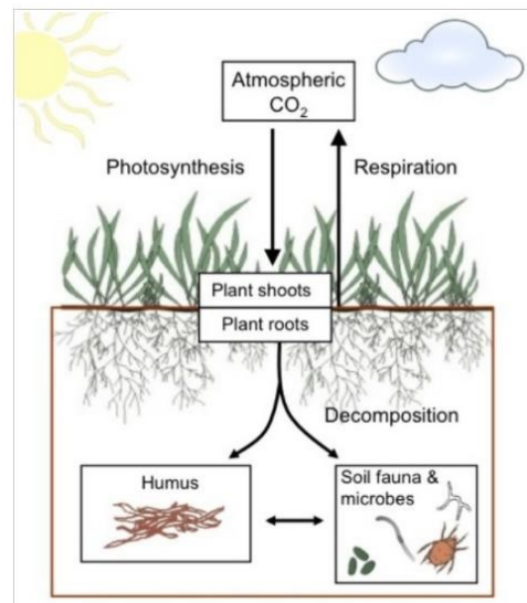
Simple diagram of air/plant/soil carbon movement ©2012 Nature Education All rights reserved.
